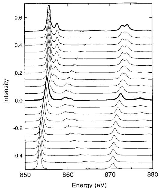
Figure 12. Series of charge-transfer multiplet calculations for the ground state 3d^8 + 3d^9 L . The top spectrum has a charge-transfer energy \Delta of +10 eV and relates to an almost pure 3d^8 state; the bottom spectrum has a value of \Delta of -10 eV and relates to an almost pure 3d^9 L state.
