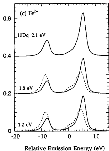
Figure 17. Theoretical spin-polarized 1s2p X-ray-emission spectra of \text{Fe}^{\text{II}} using the ligand-field multiplet calculation. Plotted are spin-down (—) and spin-up spectra (---). (Reprinted with permission from ref 121. Copyright 1997 American Physical Society.)
