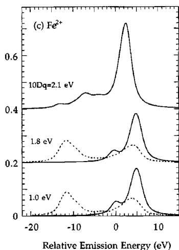
Figure 18. Theoretical spin-polarized 1s3p X-ray-emission spectra of \text{Fe}^{\text{II}} using the ligand-field multiplet calculation. Plotted are spin-down (—) and spin-up spectra (---). (Reprinted with permission from ref 121. Copyright 1997 American Physical Society.)
